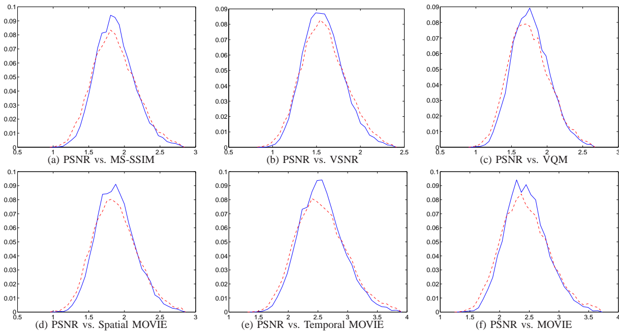
Fig. 6: Sampling distribution of the F-ratio obtained using bootstrap simulations for the F-test based on average quality scores. Sampling distributions are shown for all VQA models that are statistically superior to PSNR on the entire LIVE Video Quality Database. Note that the sampling distributions are shifted to the right of 1. Also shown in dotted lines is the sampling distribution of the F-ratio when random samples are generated to exactly satisfy the assumptions of the F-test. Note that the sampling distribution obtained from the data and the sampling distribution obtained from simulated data that satisfy the F-test assumptions are very similar.
