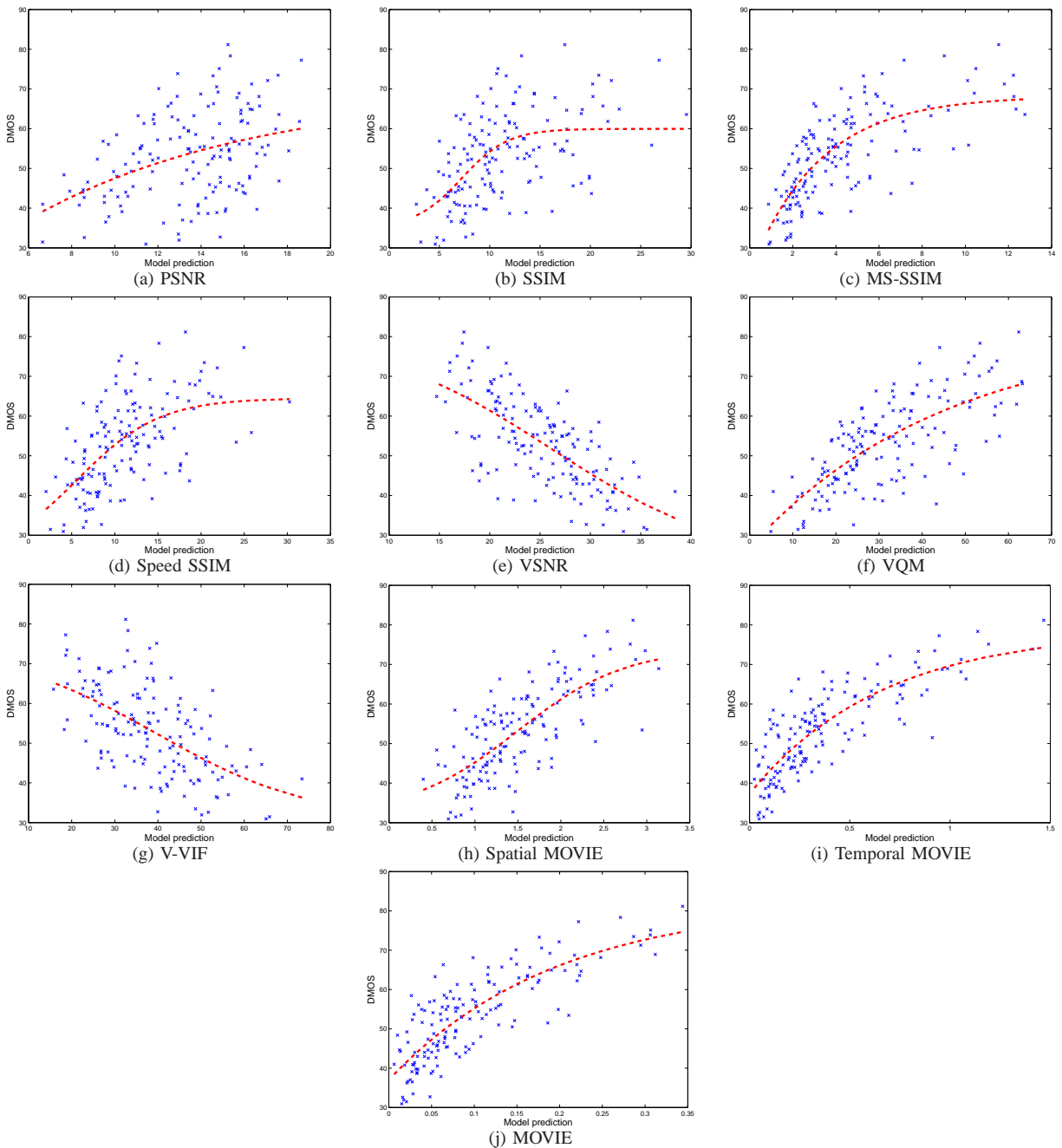
Fig. 5: Scatter plots of objective VQA scores vs. DMOS for all videos in the LIVE Video Quality Database. Also shown is the best fitting logistic function.
