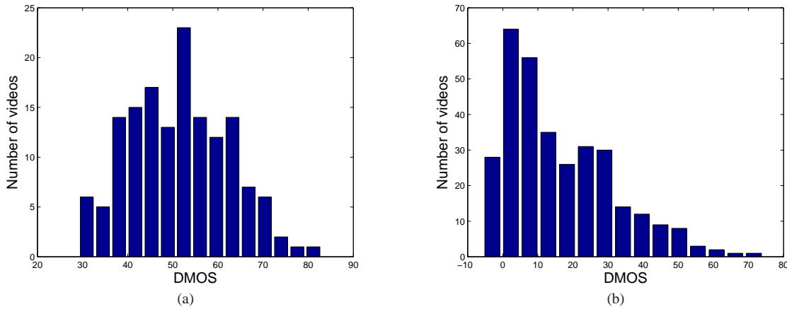
Fig. 4: Histogram of the DMOS scores in fifteen equally spaced bins between the minimum and maximum DMOS values for (a) LIVE Video Quality Database and (b) VQEG FRTV Phase 1 Database
